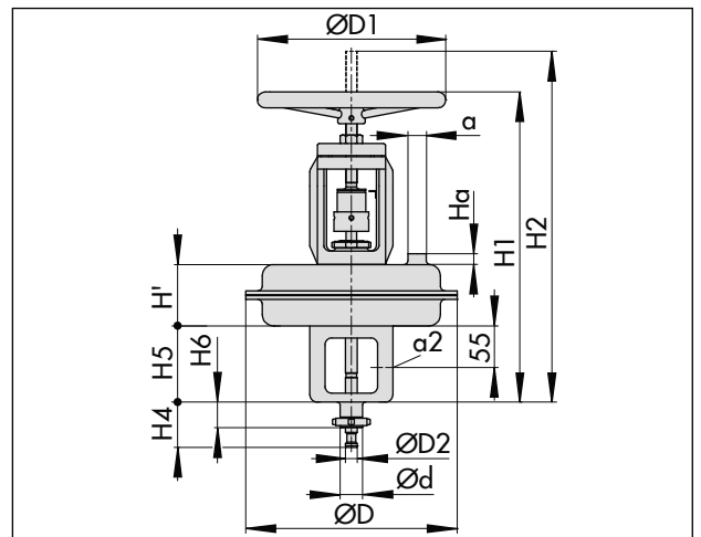
Fig. 24: Type 3277 with additional handwheel
