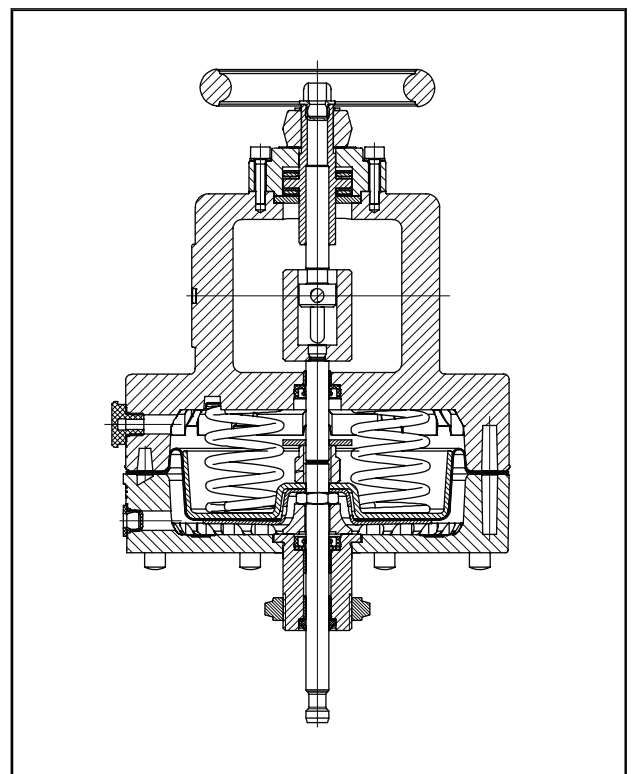
Fig. 12: Type 3271-5, "actuators stem extends" fail-safe action, with additional handwheel
