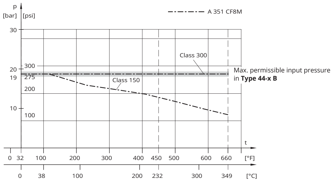
Fig. 7: Pressure-temperature diagrams for Type 44-x B with ANSI materials
